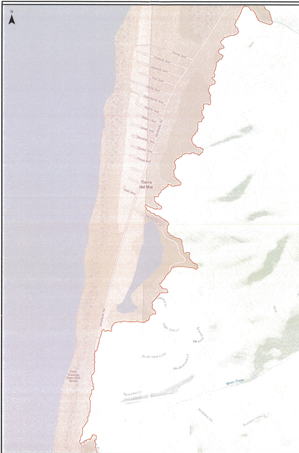
TIERRA DEL MAR TSUNAMI INUNDATION ZONE: DOGAMI TIM XXL (100% potential variability CSZ)
