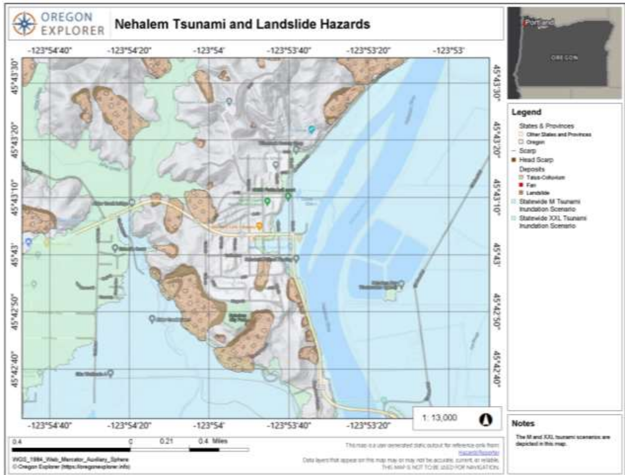
Figure 105. Nehalem Tsunami and Landslide Hazards
