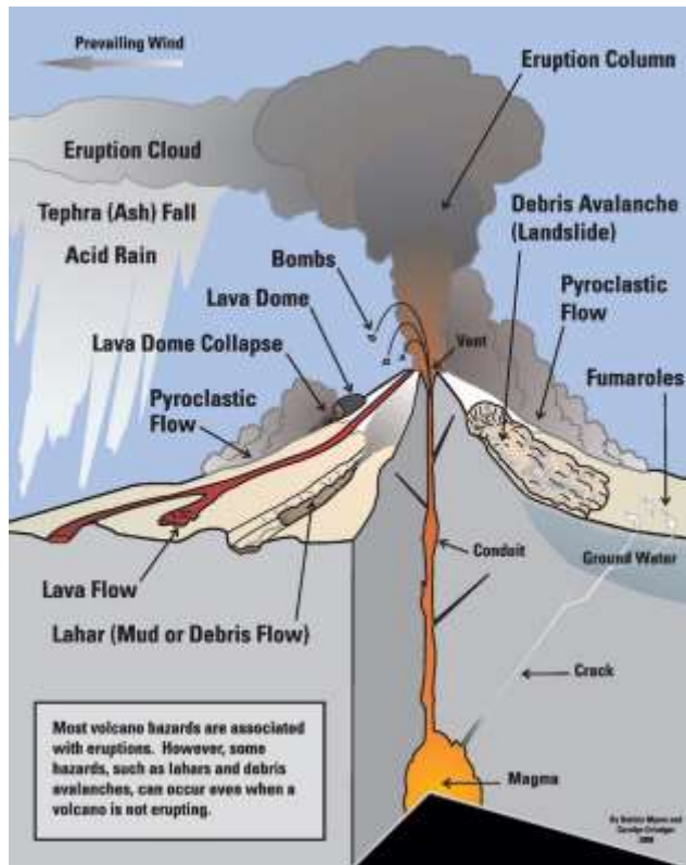
Figure 77. Potential Hazards at a Stratovolcano
