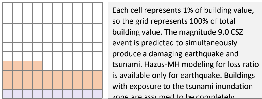
Figure 86. Loss Ratio from CSZ Event: Unincorporated Tillamook County
