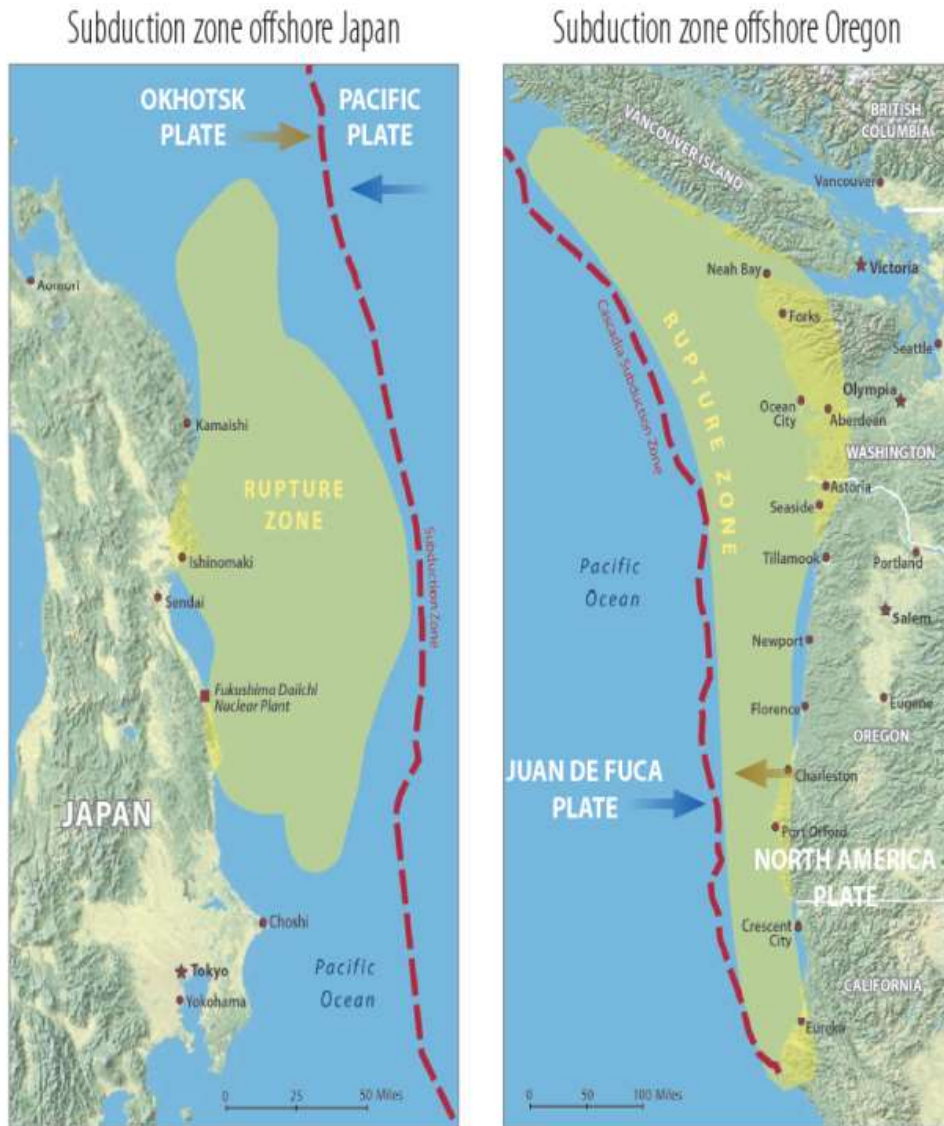
Figure 38. Comparison of the Northern Japan Subduction Zone in and the Cascadia Subduction Zone
