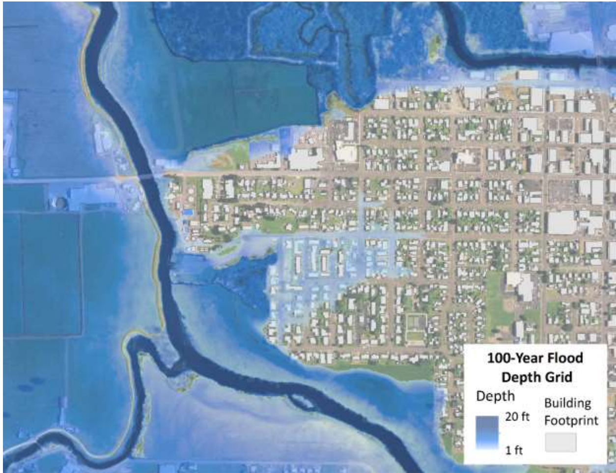
Figure 55. Flood Depth Grid Example, City of Tillamook
