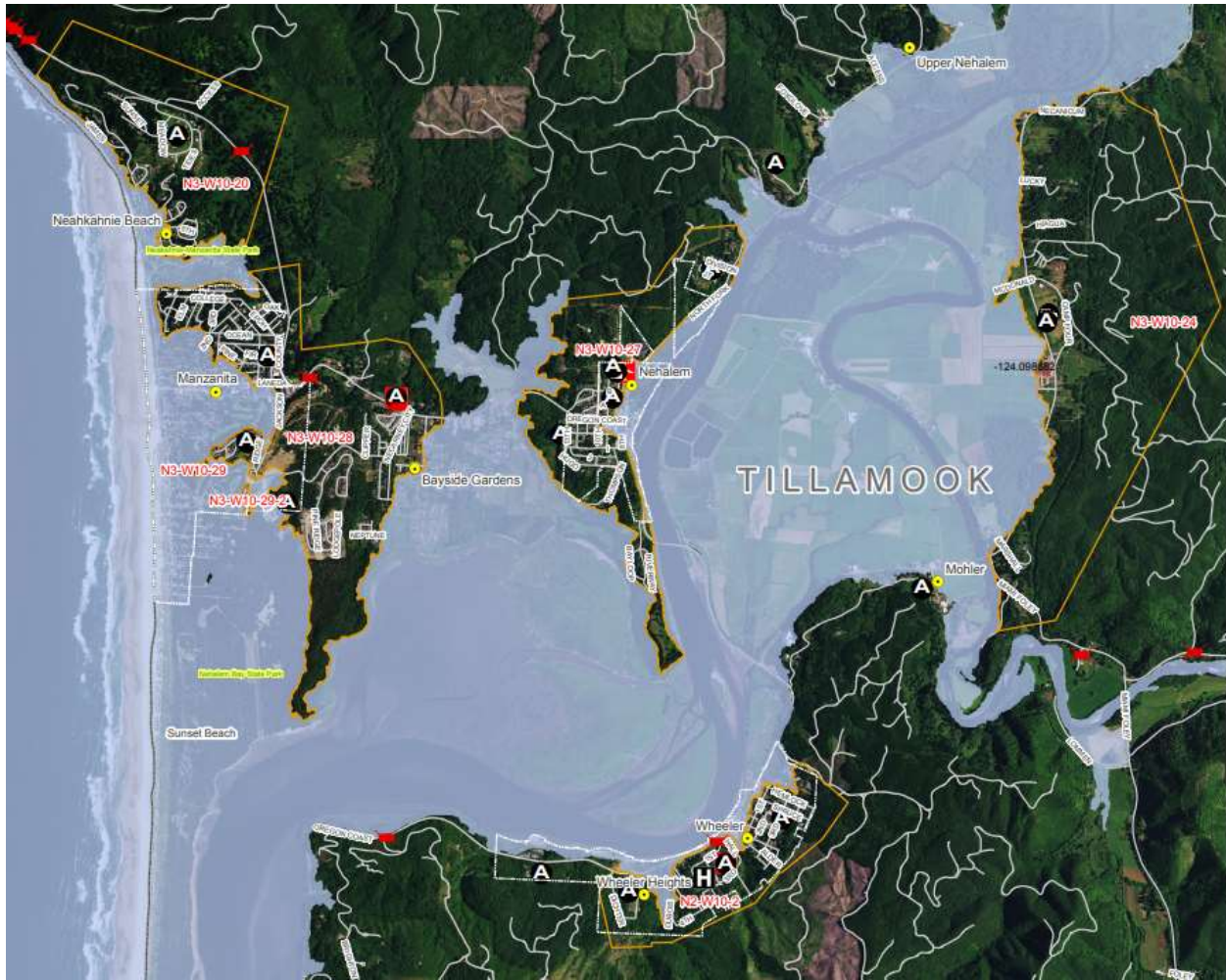
Figure 102. Cascadia Island Mapping for Manzanita, Nehalem, and Wheeler
