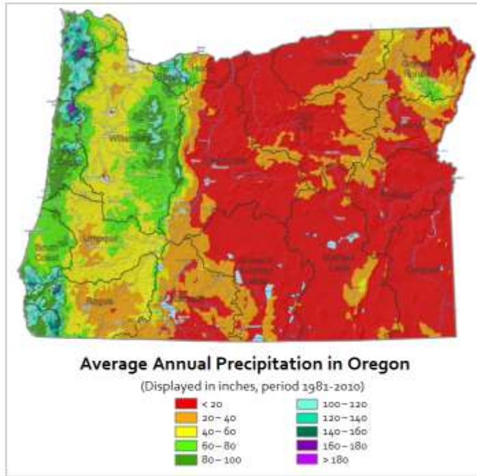
Figure 66. Oregon Average Annual Precipitation, 1981–2010
