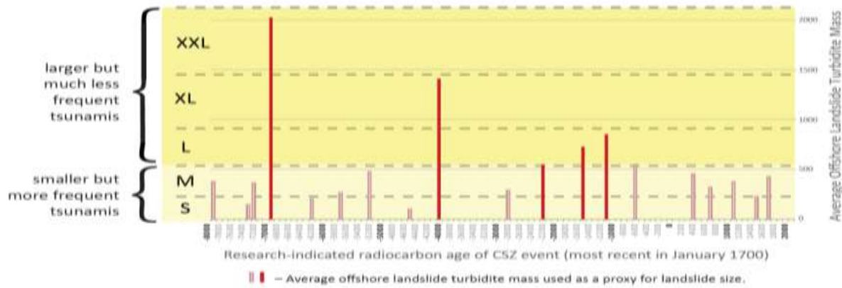
Figure 74. Occurrence and Relative Size of Cascadia Subduction Zone Megathrust Earthquakes
