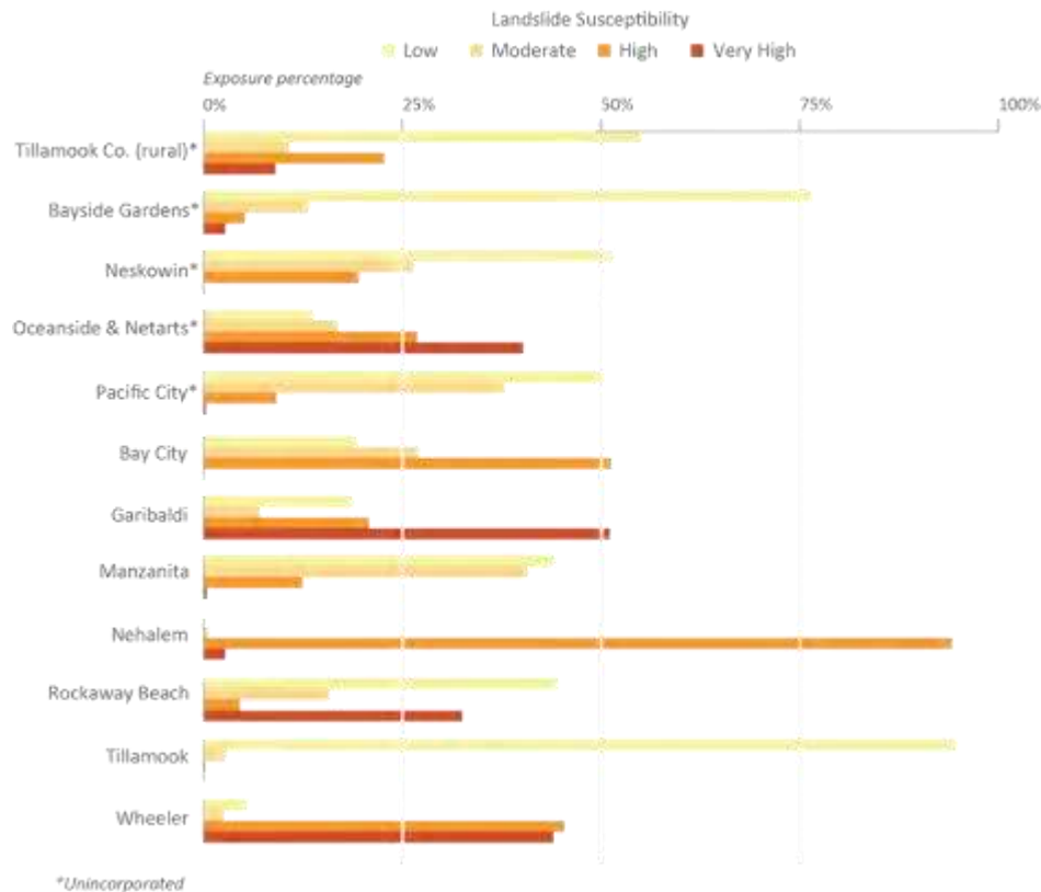
Figure 65. Landslide Susceptibility and Building Exposure Example
