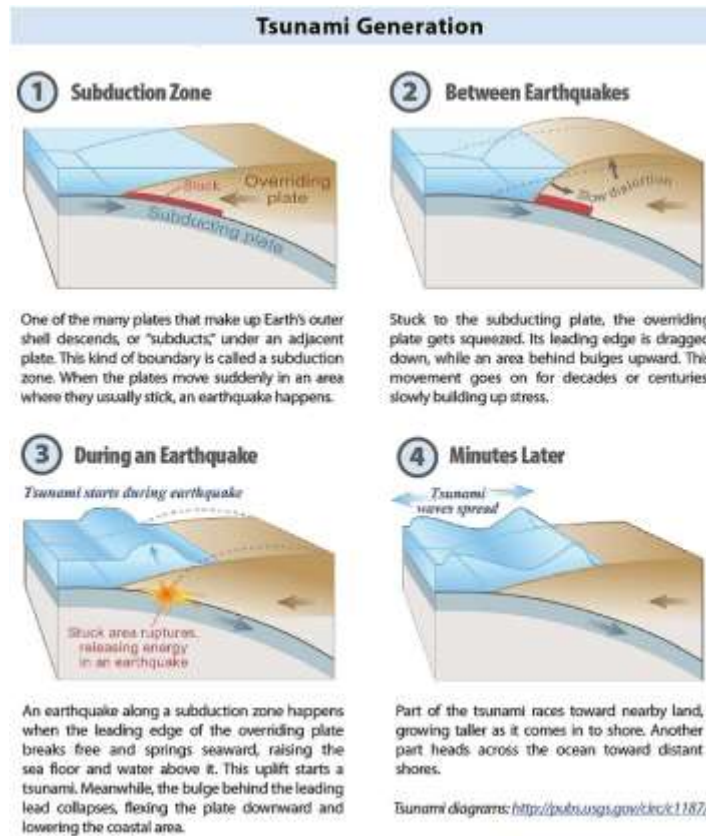
Figure 71. Generation of a Tsunami by Subduction Zone Earthquakes
