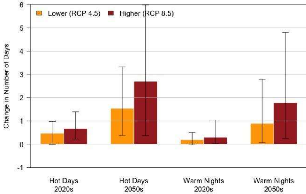
Figure 67. Change in Number of Extreme Heat Days in Tillamook County
