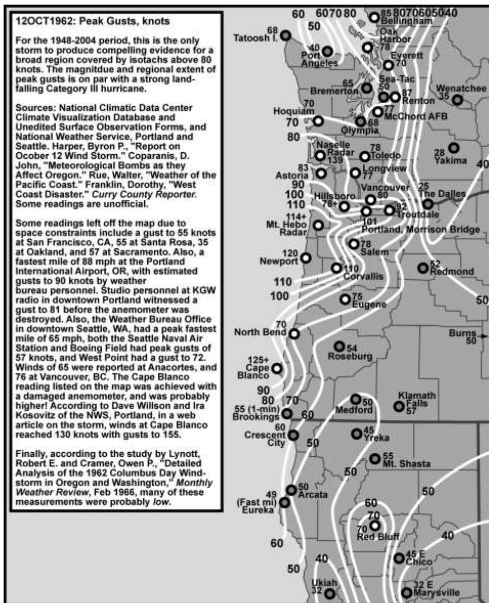
Figure 69. Peak Gusts for Windstorm on October 12, 1962
