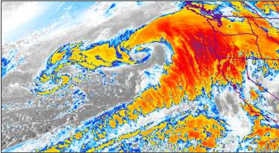
Figure 68. Satellite Image of the Type of Severe Pacific Storm that Can Bring High Winds to Western Oregon
