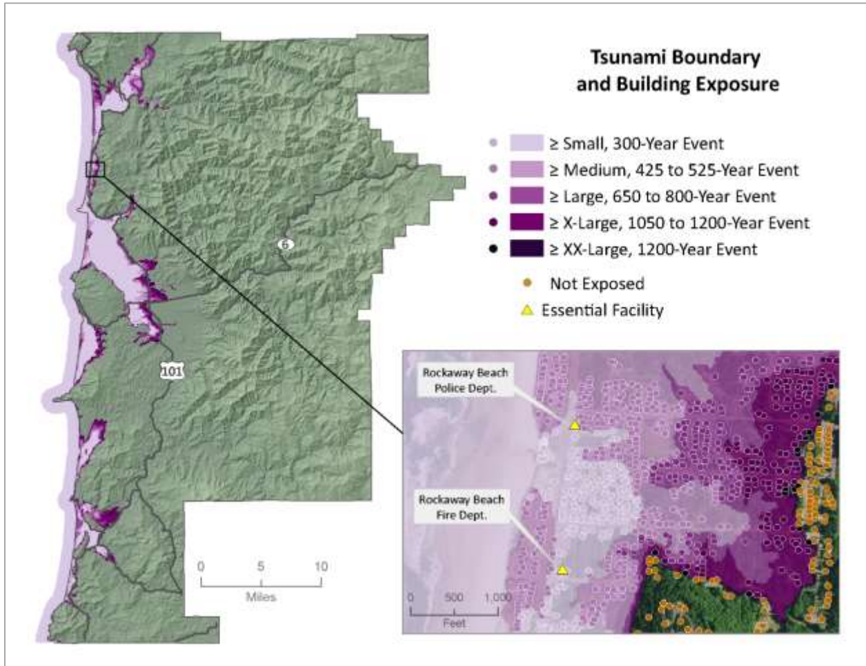
Figure 75. Tsunami Inundation Scenarios and Building Exposure Example
